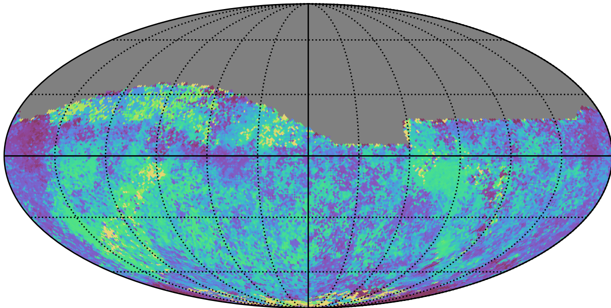
noroll_mjdp365_v3.4_10yrs Yr 1 all bands: Median skyBrightness
