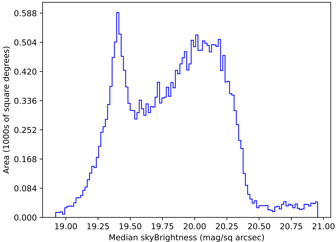
noroll_mjdp365_v3.4_10yrs Yr 1 all bands: Median skyBrightness
