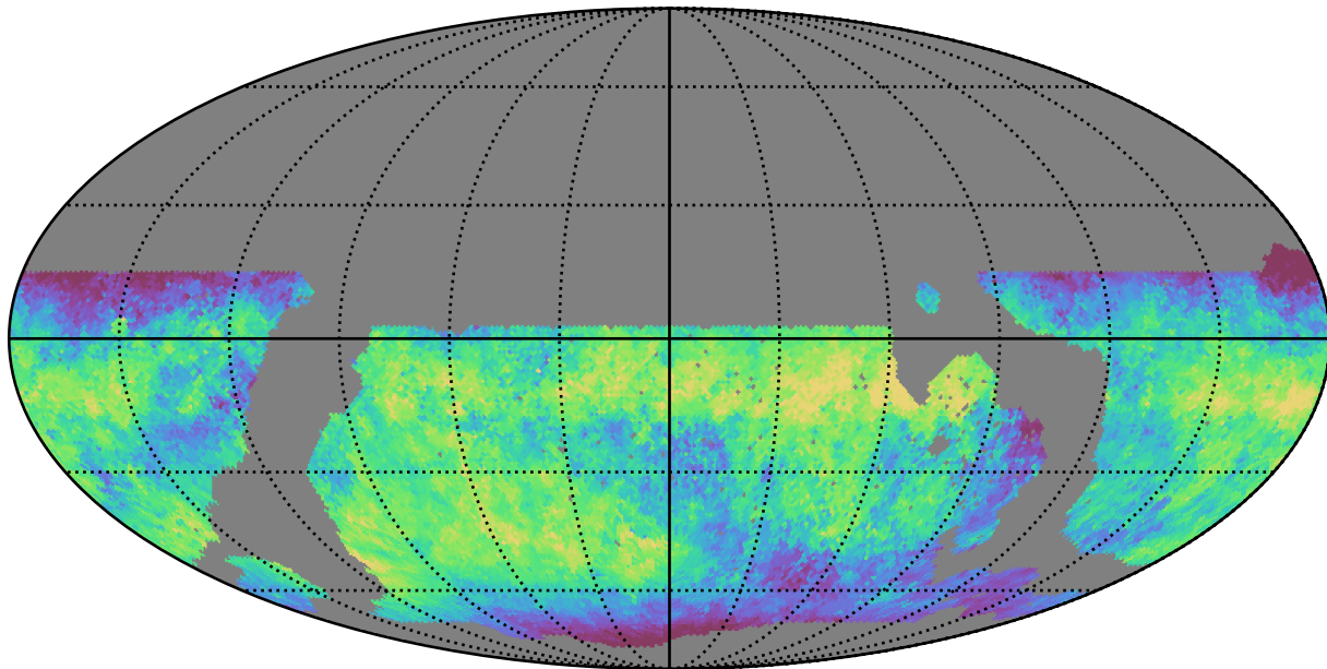
noroll_mjdp365_v3.4_10yrs WFD z band: Median skyBrightness
