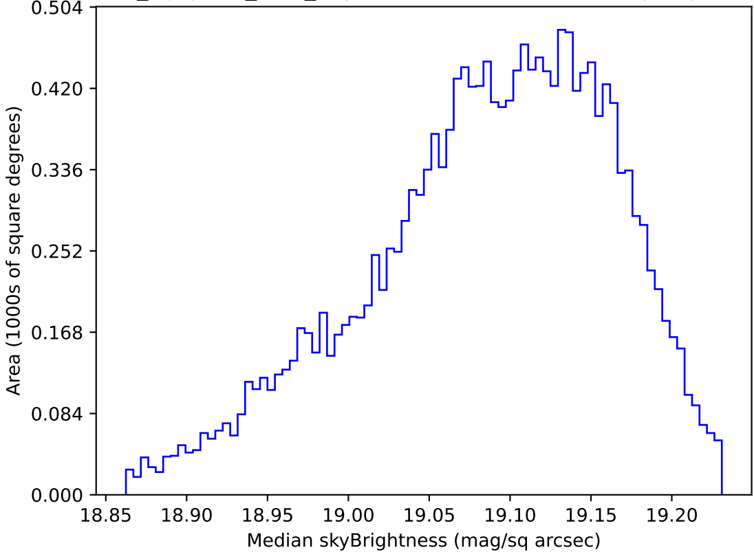
noroll_mjdp365_v3.4_10yrs WFD z band: Median skyBrightness
