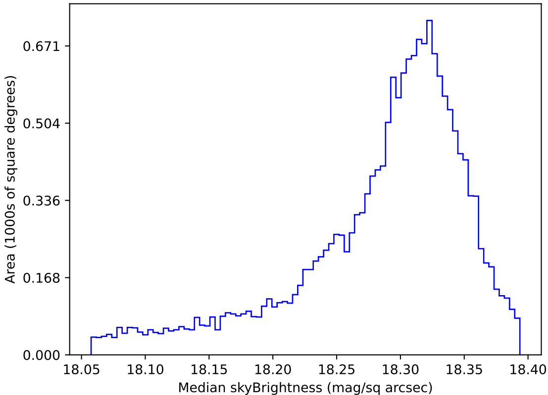
noroll_mjdp365_v3.4_10yrs WFD y band: Median skyBrightness
