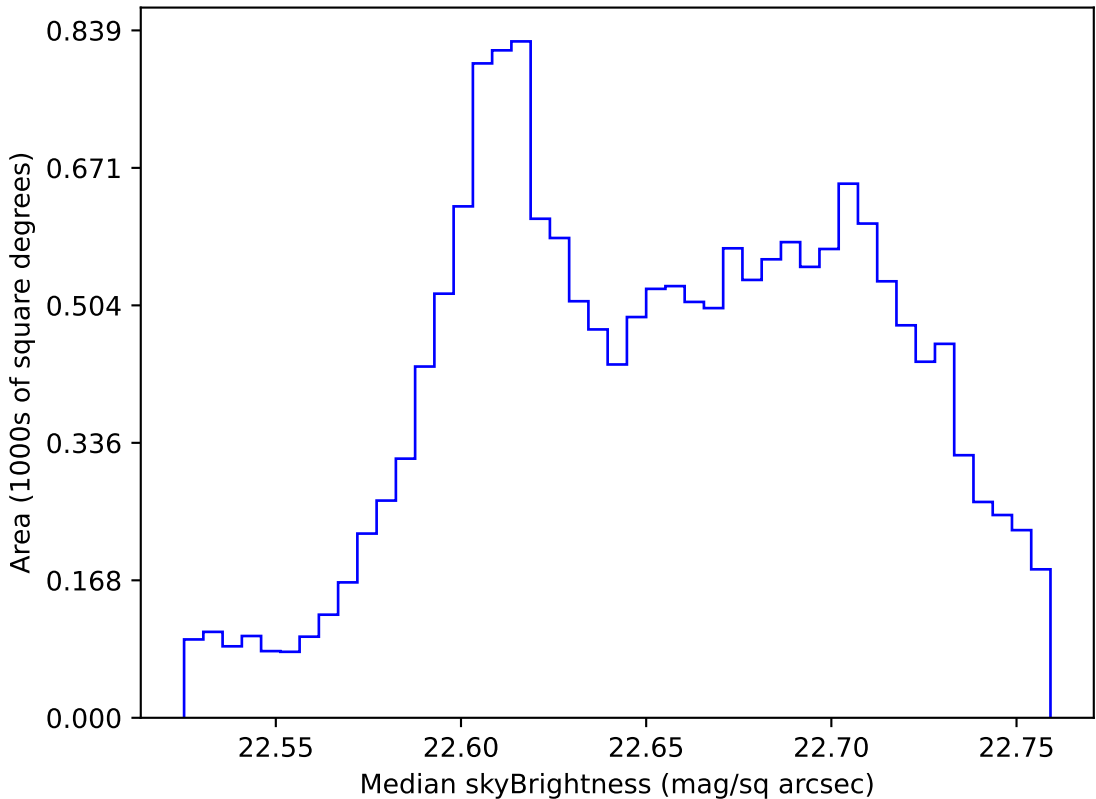
noroll_mjdp365_v3.4_10yrs WFD u band: Median skyBrightness
