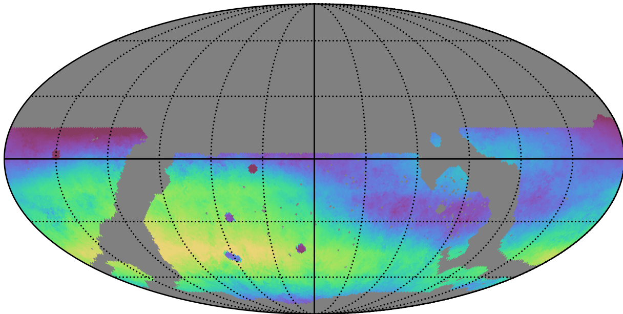
noroll_mjdp365_v3.4_10yrs WFD r band: Median skyBrightness
