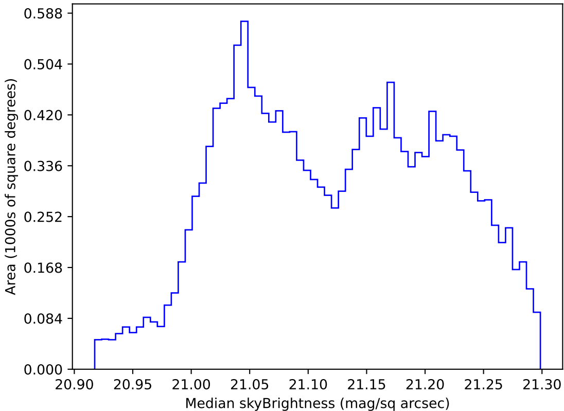
noroll_mjdp365_v3.4_10yrs WFD r band: Median skyBrightness
