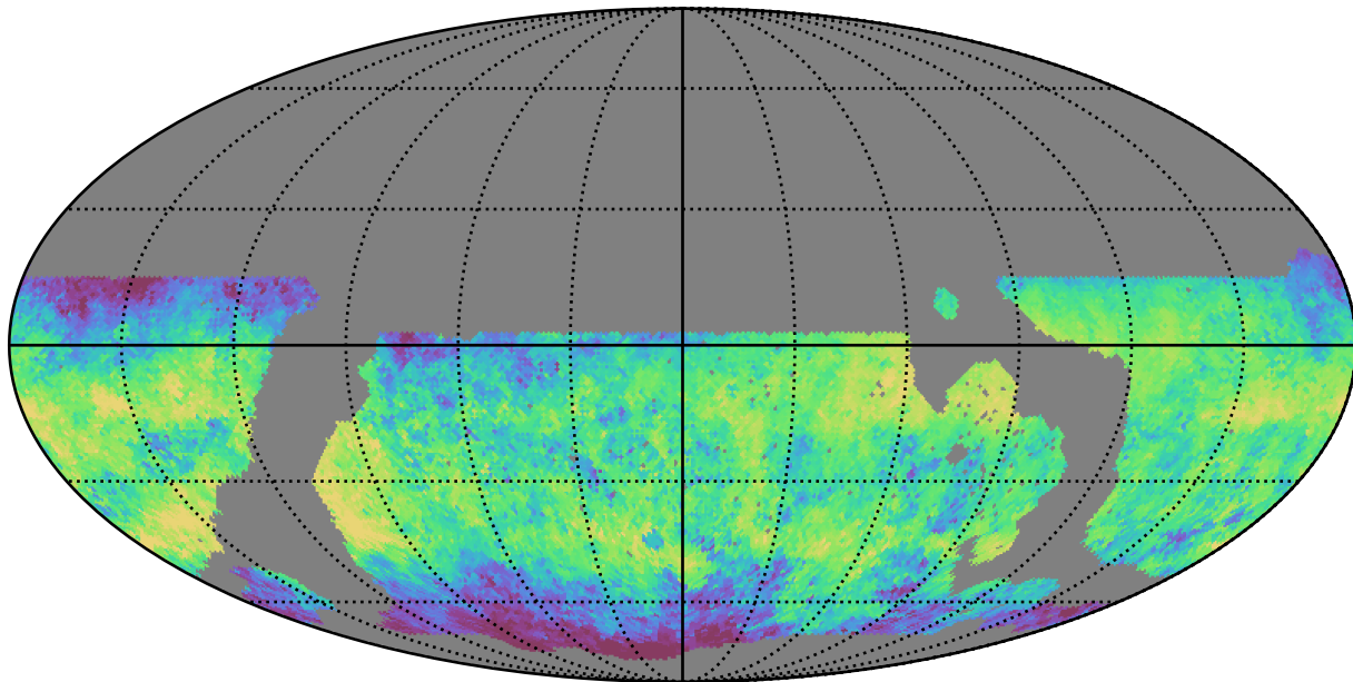
noroll_mjdp365_v3.4_10yrs WFD i band: Median skyBrightness
