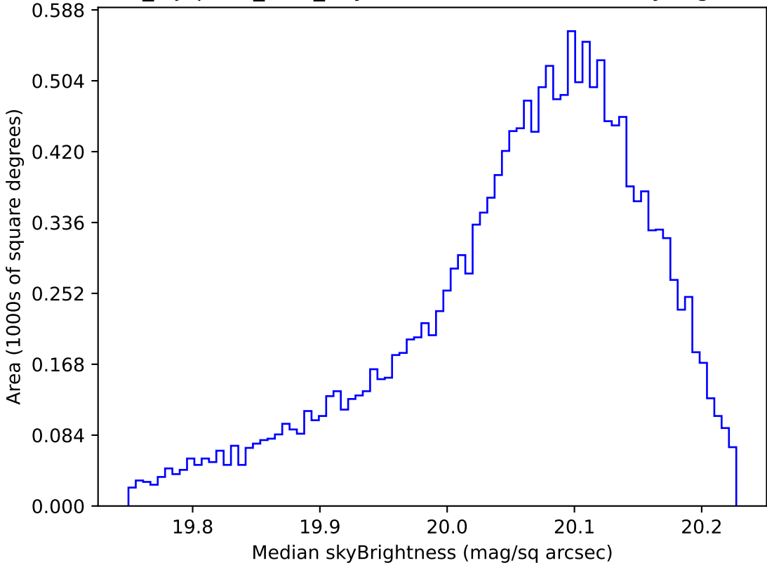
noroll_mjdp365_v3.4_10yrs WFD i band: Median skyBrightness
