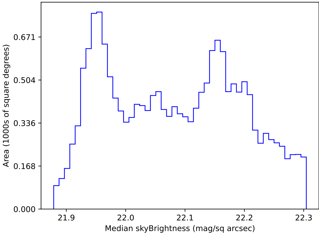
noroll_mjdp365_v3.4_10yrs WFD g band: Median skyBrightness
