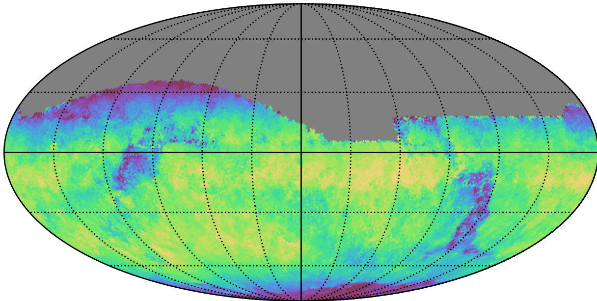
noroll_mjdp365_v3.4_10yrs All sky z band: Median skyBrightness
