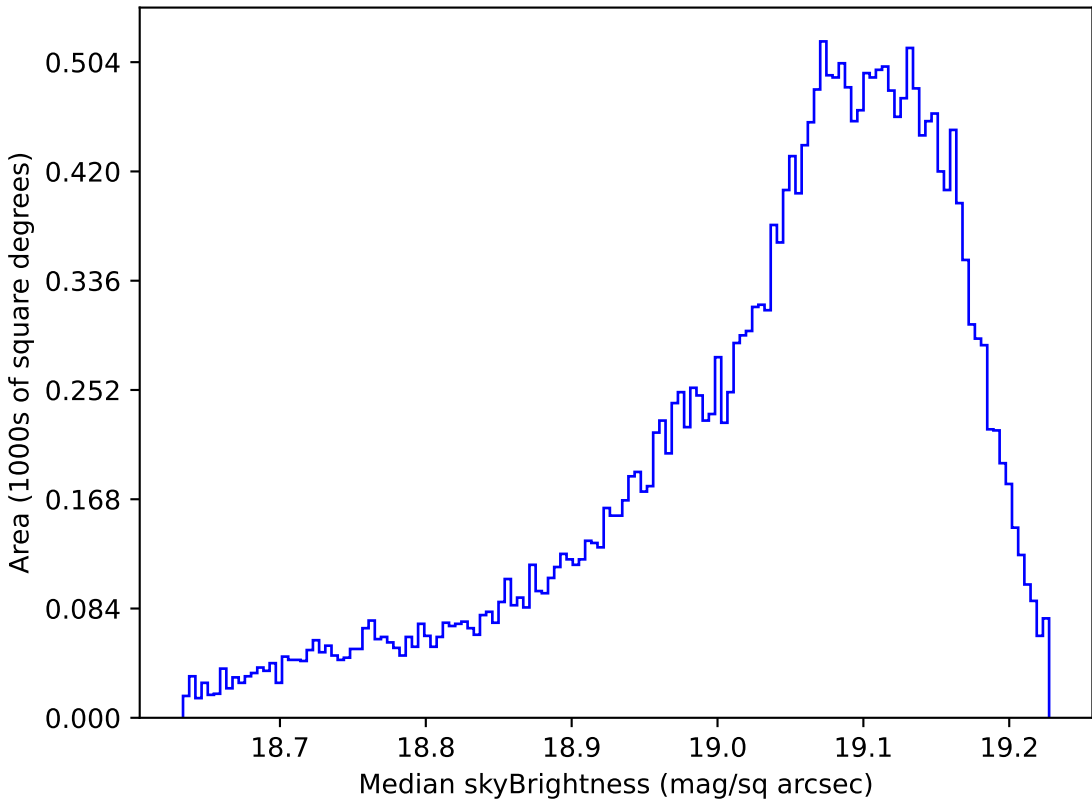
noroll_mjdp365_v3.4_10yrs All sky z band: Median skyBrightness
