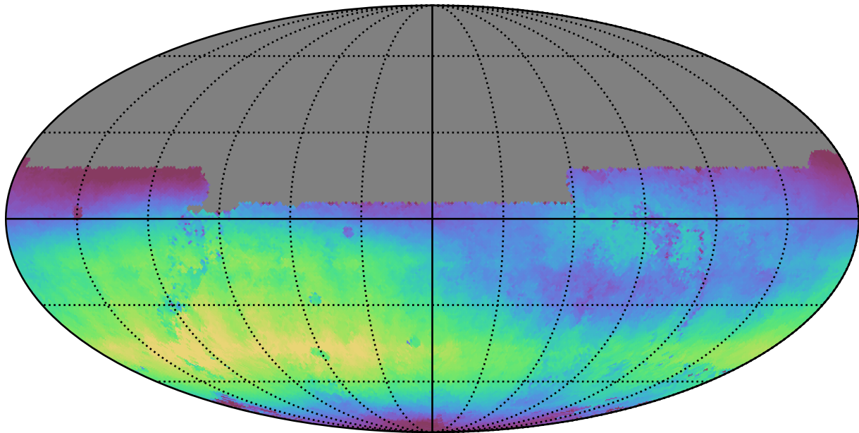
noroll_mjdp365_v3.4_10yrs All sky u band: Median skyBrightness
