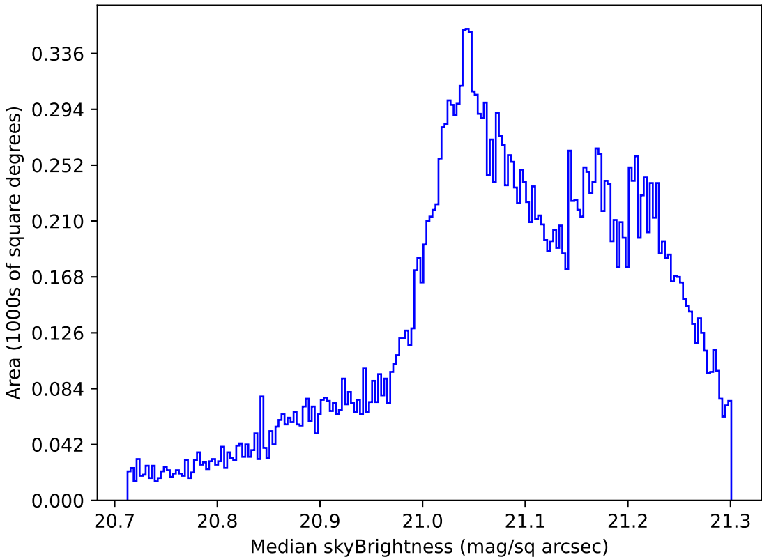
noroll_mjdp365_v3.4_10yrs All sky r band: Median skyBrightness
