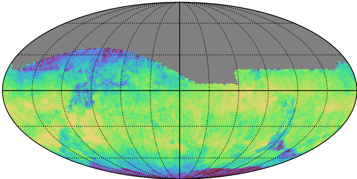
noroll_mjdp365_v3.4_10yrs All sky i band: Median skyBrightness
