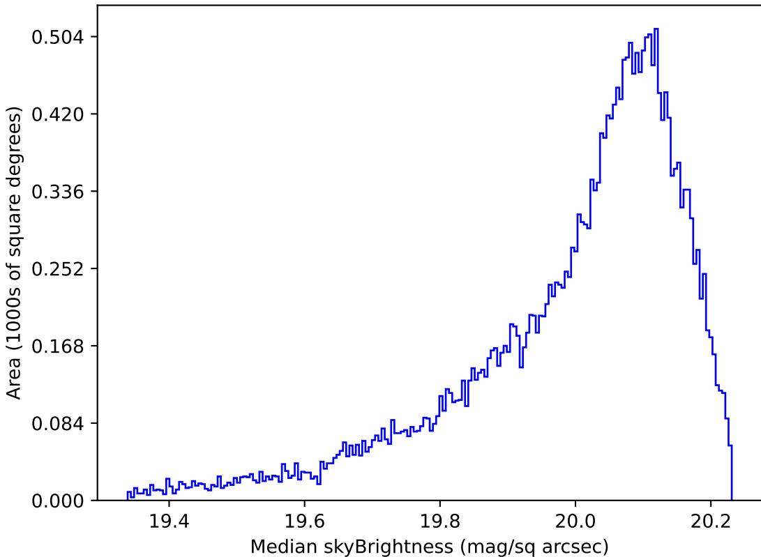
noroll_mjdp365_v3.4_10yrs All sky i band: Median skyBrightness
