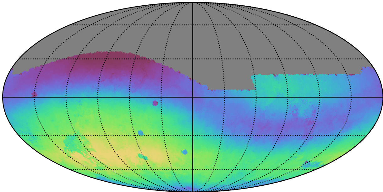
noroll_mjdp365_v3.4_10yrs All sky g band: Median skyBrightness
