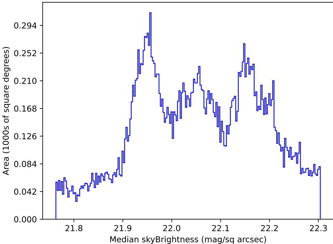
noroll_mjdp365_v3.4_10yrs All sky g band: Median skyBrightness
