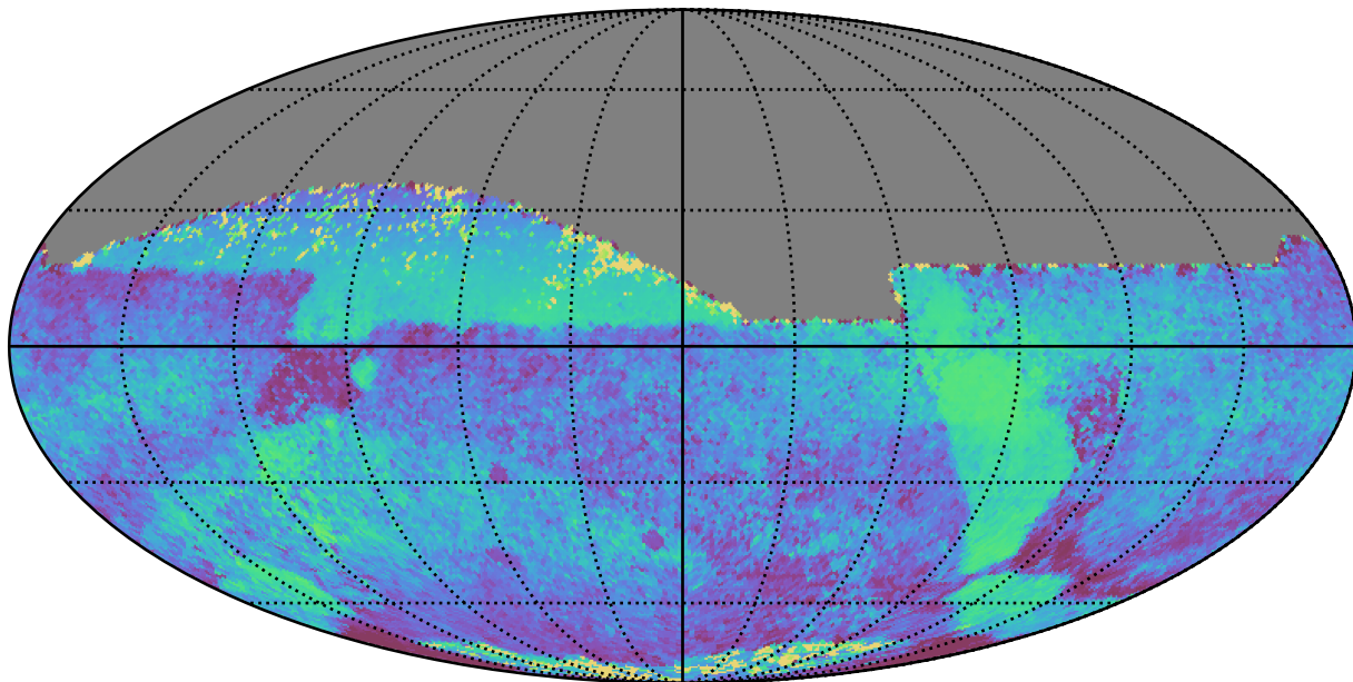
noroll_mjdp365_v3.4_10yrs All sky all bands: Median skyBrightness
