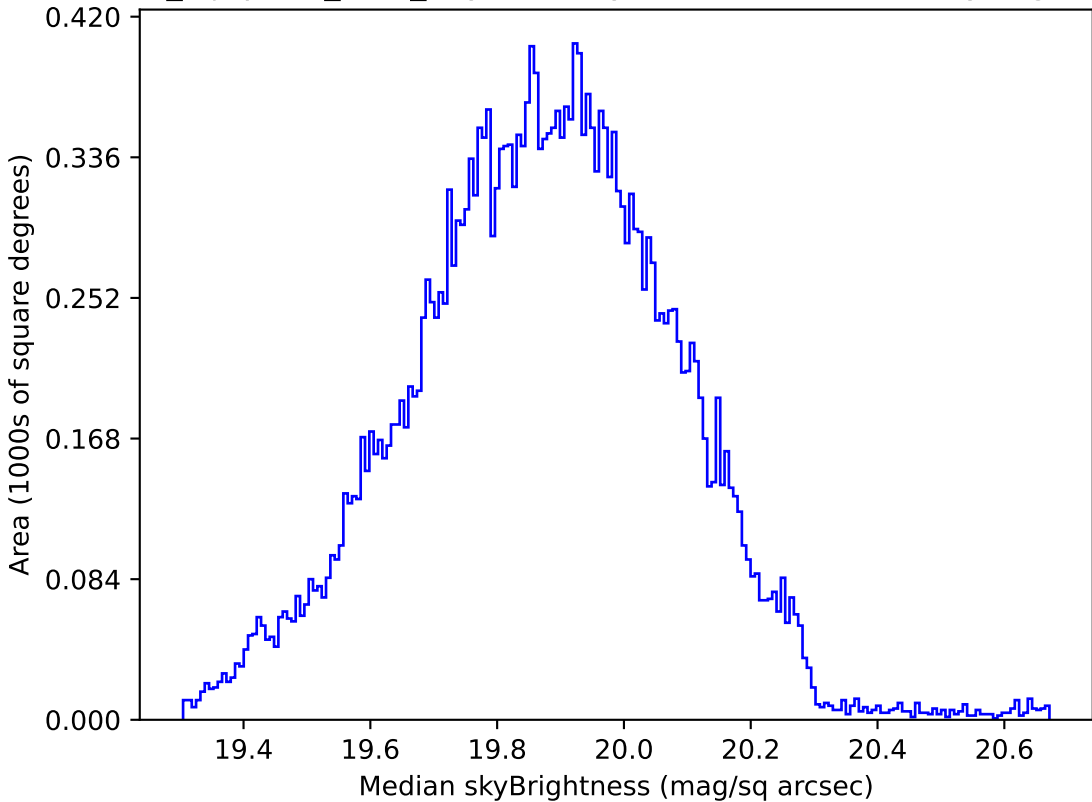
noroll_mjdp365_v3.4_10yrs All sky all bands: Median skyBrightness
