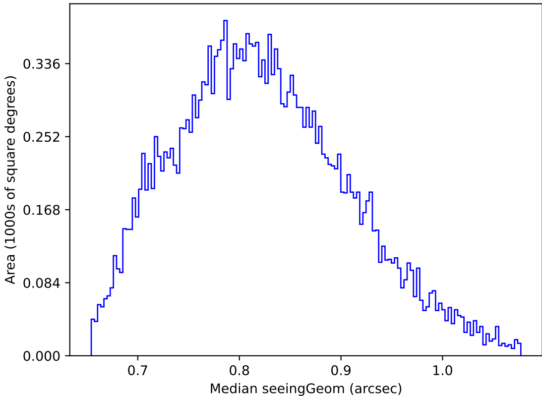
noroll_mjdp365_v3.4_10yrs Yr 1 y band: Median seeingGeom
