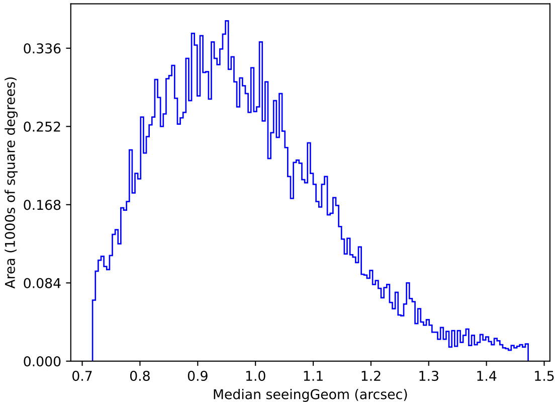
noroll_mjdp365_v3.4_10yrs Yr 1 u band: Median seeingGeom
