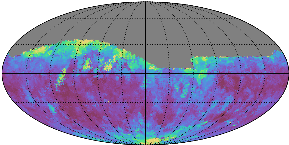
noroll_mjdp365_v3.4_10yrs Yr 1 r band: Median seeingGeom
