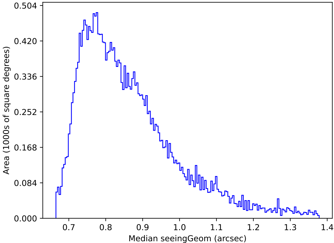
noroll_mjdp365_v3.4_10yrs Yr 1 r band: Median seeingGeom
