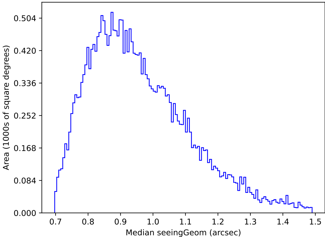
noroll_mjdp365_v3.4_10yrs Yr 1 g band: Median seeingGeom
