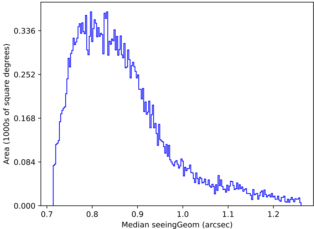
noroll_mjdp365_v3.4_10yrs Yr 1 all bands: Median seeingGeom
