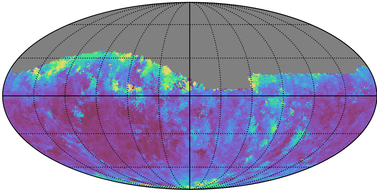
noroll_mjdp365_v3.4_10yrs Yr 1 z band: Median seeingEff
