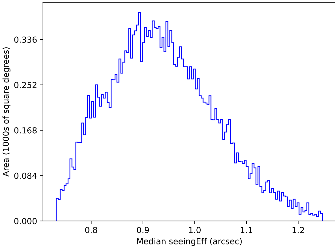
noroll_mjdp365_v3.4_10yrs Yr 1 y band: Median seeingEff
