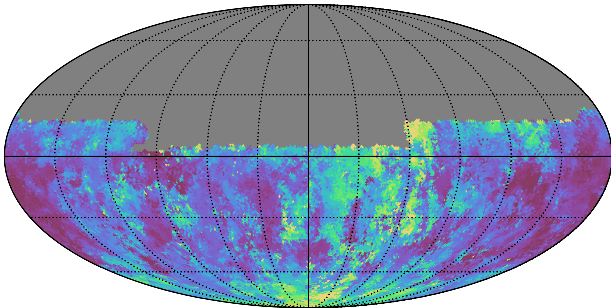
noroll_mjdp365_v3.4_10yrs Yr 1 u band: Median seeingEff
