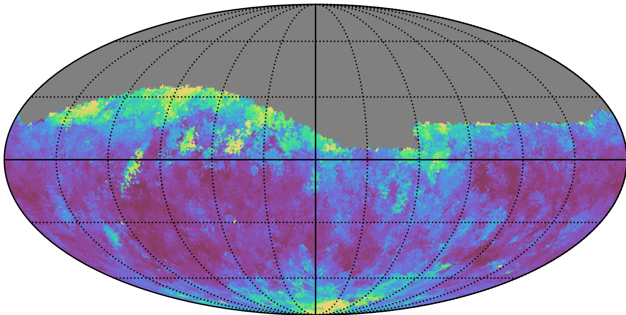
noroll_mjdp365_v3.4_10yrs Yr 1 r band: Median seeingEff
