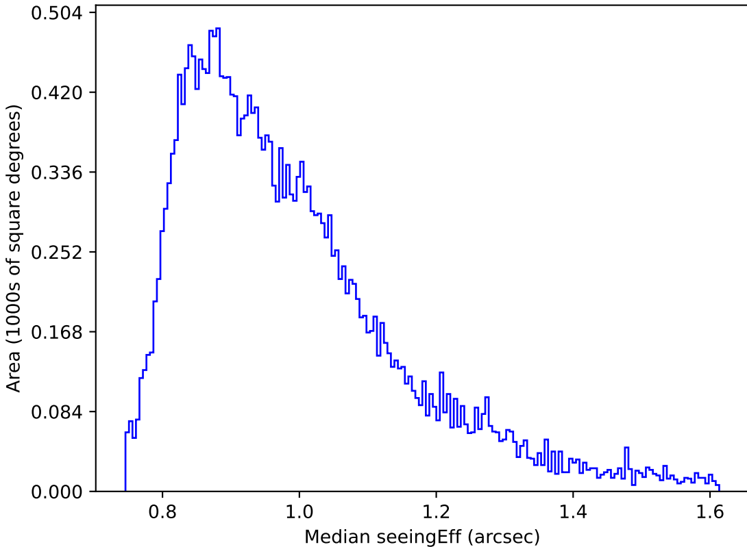
noroll_mjdp365_v3.4_10yrs Yr 1 r band: Median seeingEff
