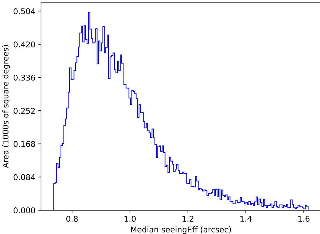
noroll_mjdp365_v3.4_10yrs Yr 1 i band: Median seeingEff
