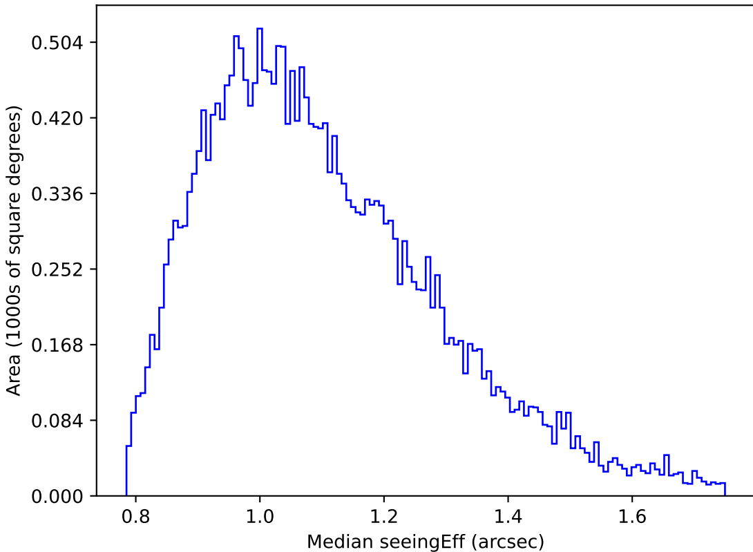
noroll_mjdp365_v3.4_10yrs Yr 1 g band: Median seeingEff
