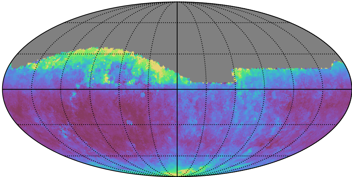
noroll_mjdp365_v3.4_10yrs Yr 1 all bands: Median seeingEff
