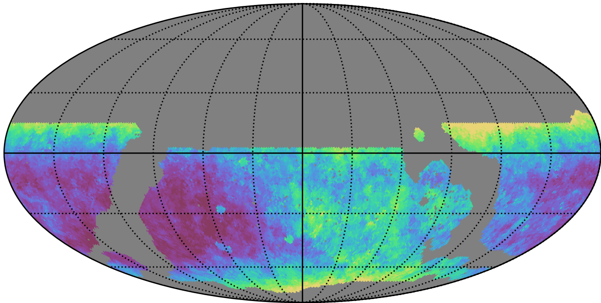
noroll_mjdp365_v3.4_10yrs WFD z band: Median seeingEff
