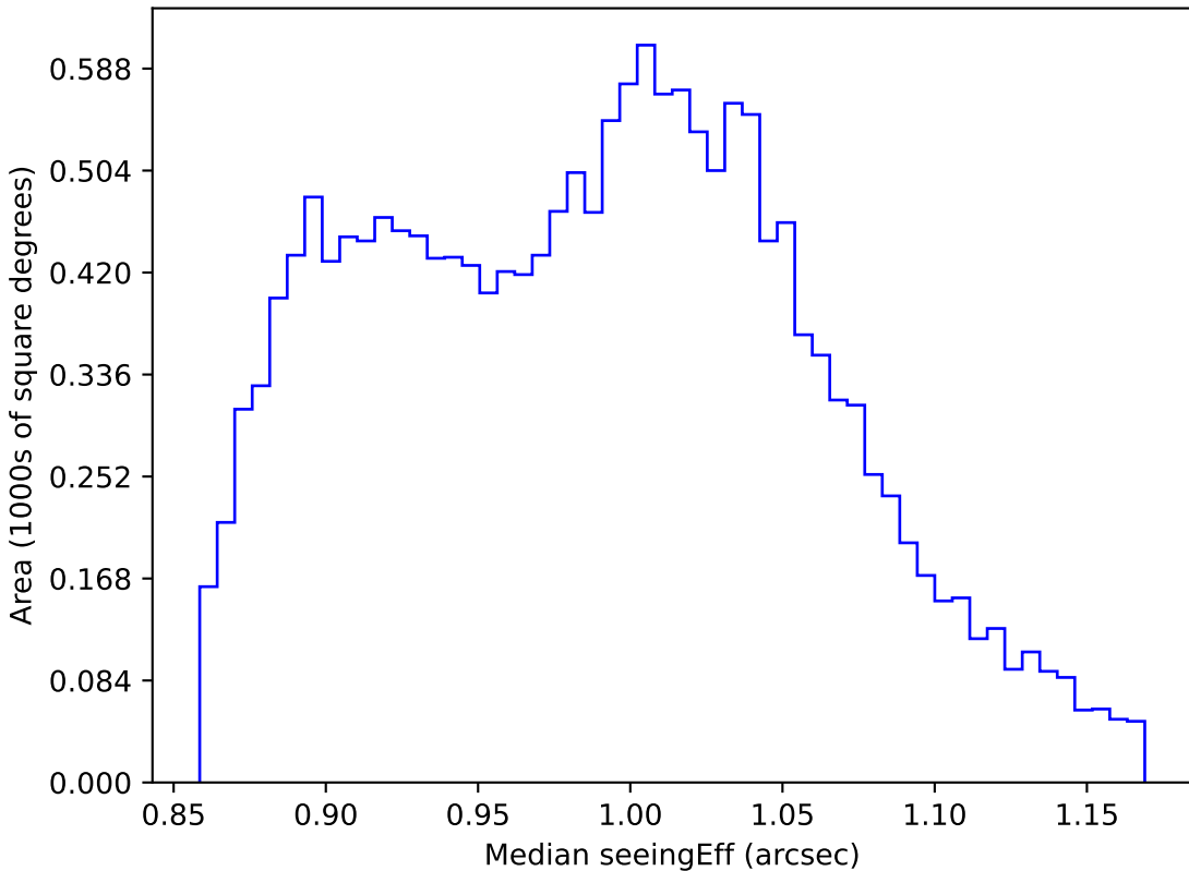
noroll_mjdp365_v3.4_10yrs WFD z band: Median seeingEff
