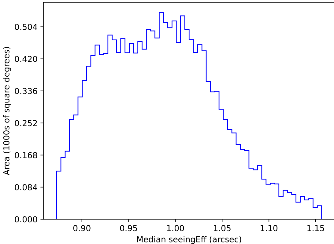
noroll_mjdp365_v3.4_10yrs WFD y band: Median seeingEff
