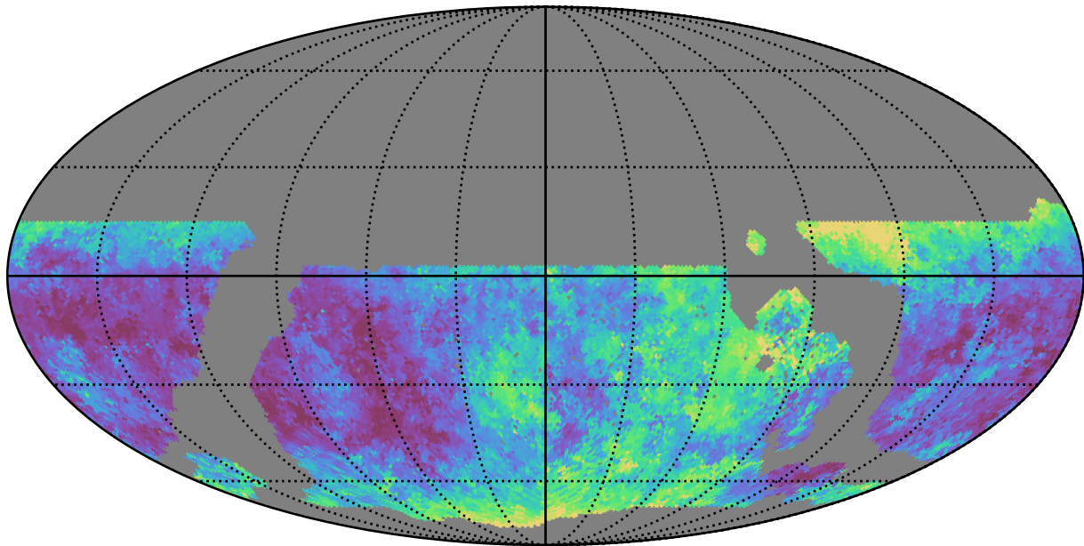
noroll_mjdp365_v3.4_10yrs WFD u band: Median seeingEff
