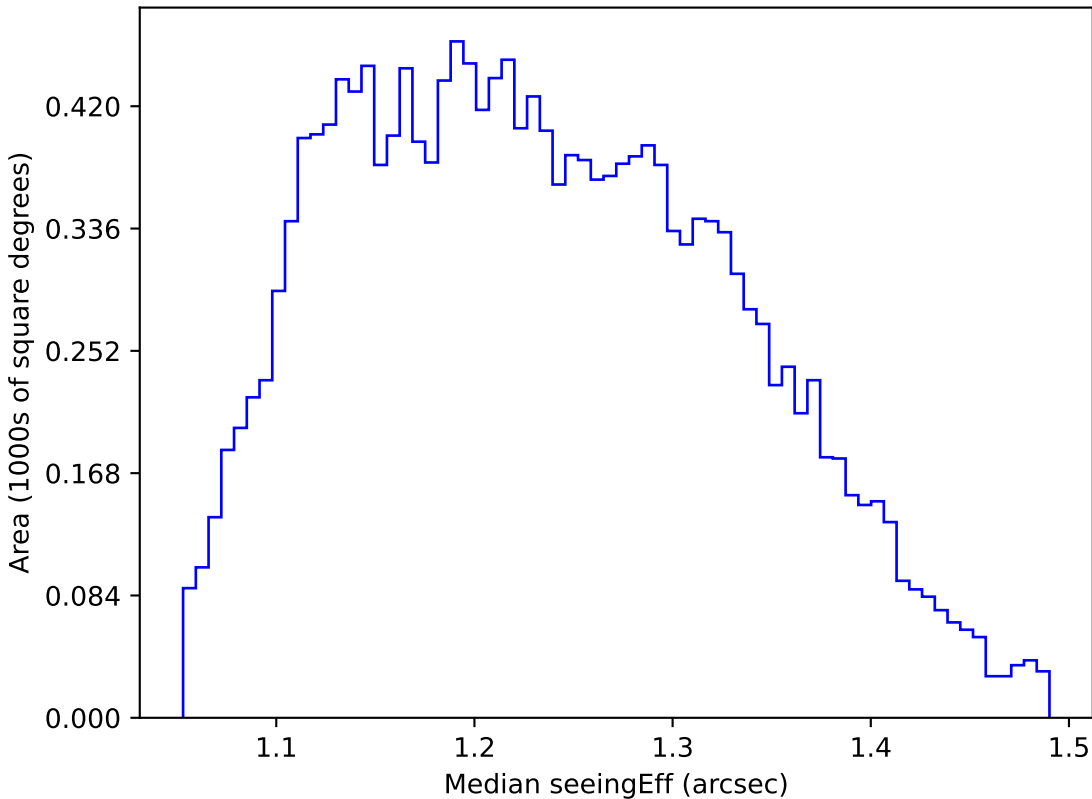
noroll_mjdp365_v3.4_10yrs WFD u band: Median seeingEff
