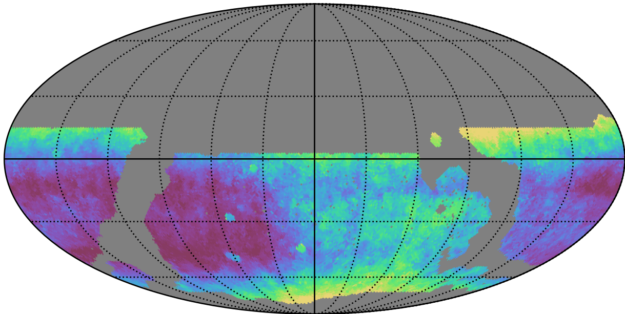
noroll_mjdp365_v3.4_10yrs WFD i band: Median seeingEff
