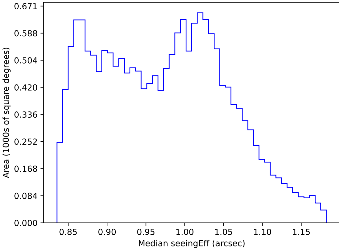
noroll_mjdp365_v3.4_10yrs WFD i band: Median seeingEff
