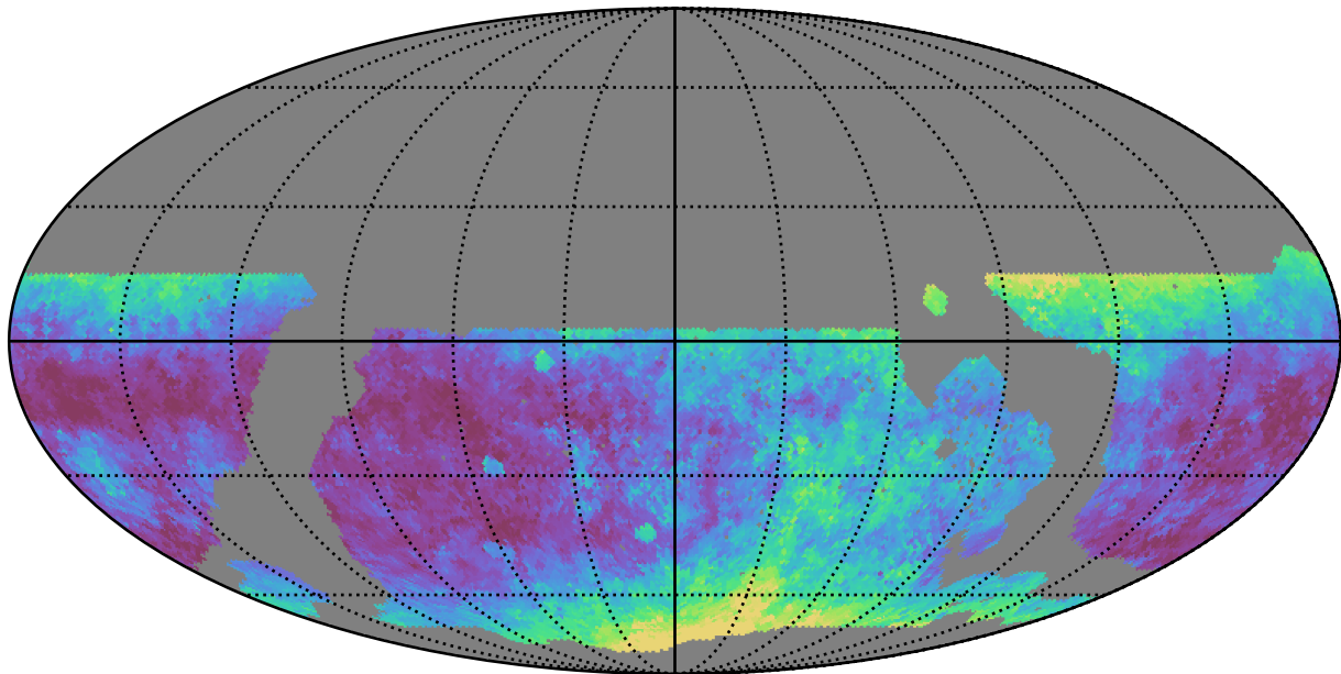
noroll_mjdp365_v3.4_10yrs WFD g band: Median seeingEff
