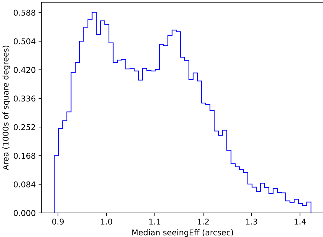
noroll_mjdp365_v3.4_10yrs WFD g band: Median seeingEff
