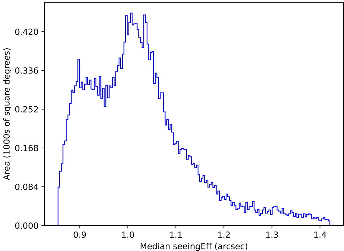
noroll_mjdp365_v3.4_10yrs All sky z band: Median seeingEff
