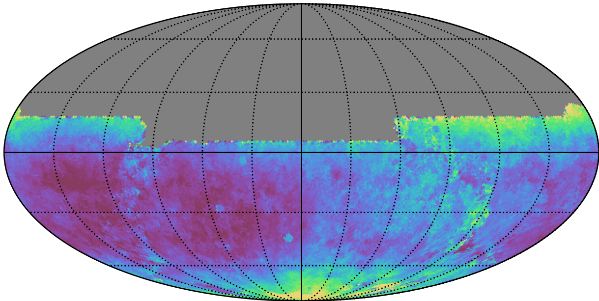
noroll_mjdp365_v3.4_10yrs All sky y band: Median seeingEff
