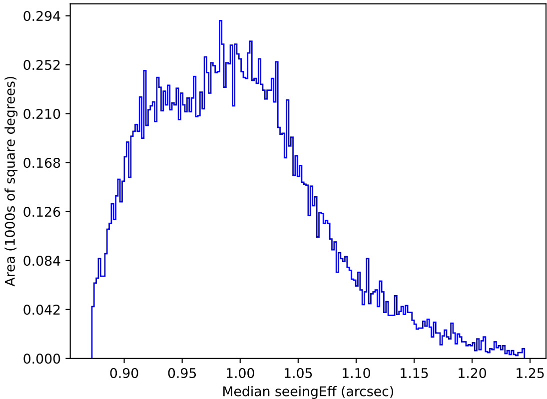
noroll_mjdp365_v3.4_10yrs All sky y band: Median seeingEff
