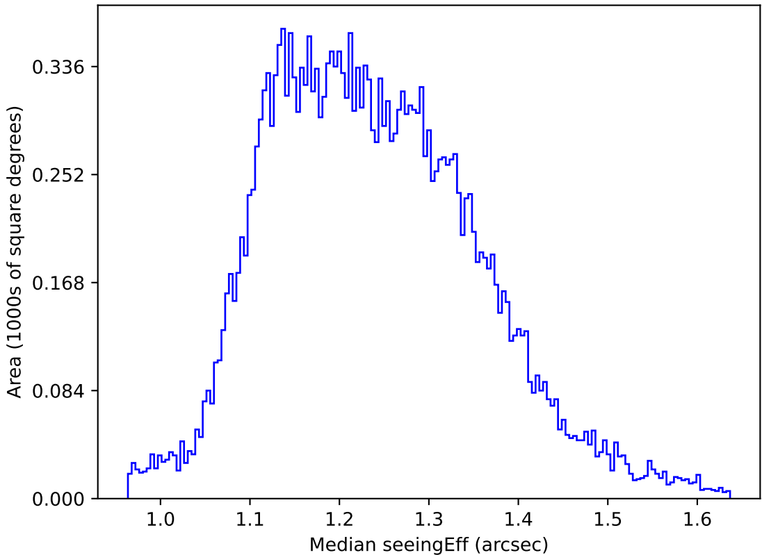
noroll_mjdp365_v3.4_10yrs All sky u band: Median seeingEff
