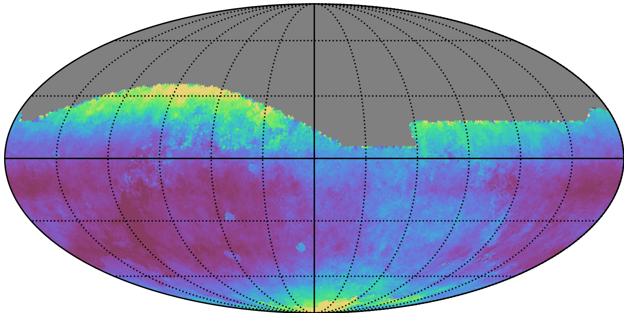
noroll_mjdp365_v3.4_10yrs All sky r band: Median seeingEff
