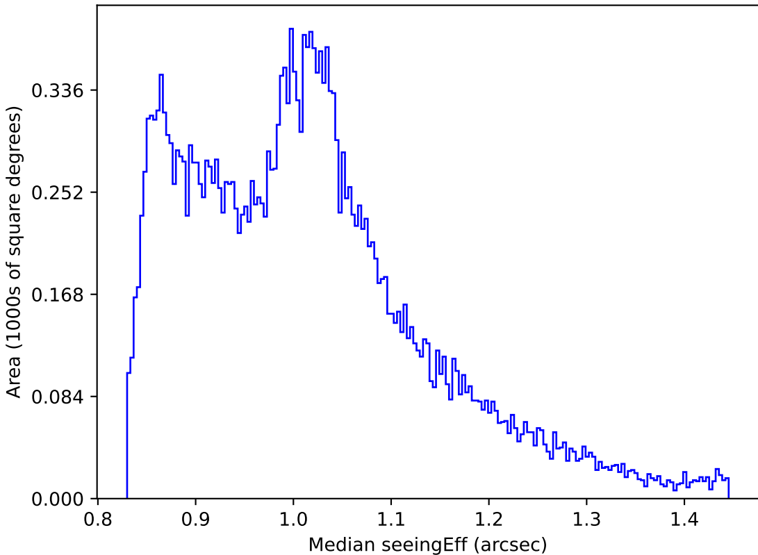
noroll_mjdp365_v3.4_10yrs All sky i band: Median seeingEff
